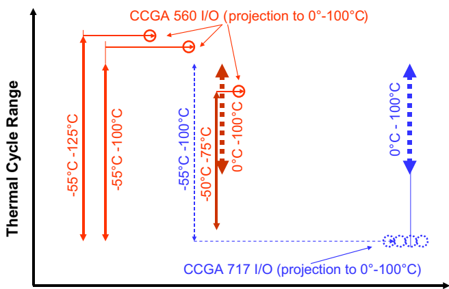
Fig. 21. Effect of temperature range on first failure for CCGA 560 I/Os and no failure yet ( -55/100\text{ }^{\circ}\text{C} ) for CCGA 717 I/Os using a modified Coffin–Manson relationship.
