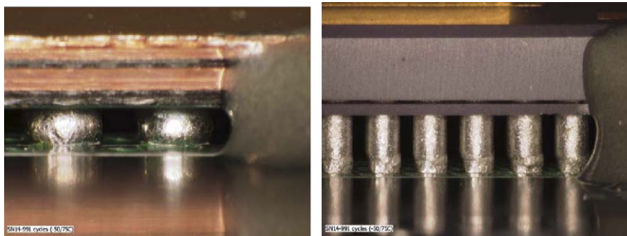
Fig. 10. Optical photomicrographs of PBGA (left) and CCGA built with a 10.5 mil thick stencil after 991 cycles Cycle A ( -50/75^{\circ}\text{C} )—corner staking adhesives apparent at the two corners.
