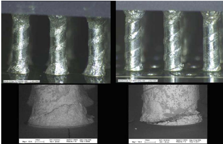
Fig. 20. Optical and SEM (bottom) photomicrographs of CCGA 717 I/O assembly at 400 thermal cycles ( -65/150\text{ }^{\circ}\text{C} ) showing signs of cracking for NSMD pad design with good solder fillet (left) and failure for SMD (right) with lack of solder fillet.
