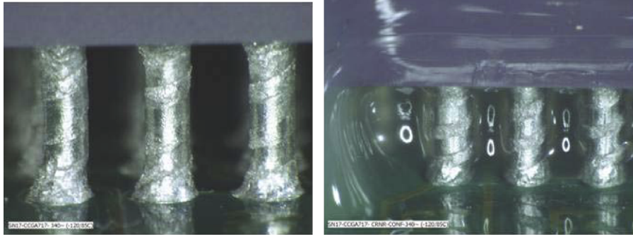
Fig. 19. Optical photomicrographs of CCGA 717 I/O assembly at 340 thermal cycles ( -120/85\text{ }^{\circ}\text{C} ) showing signs of damage, left with no conformal coat and no corner staking and right with conformal coat and corner staking.
