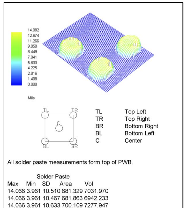
Fig. 7. Solder paste distribution using a laser profilometer showing the calculated paste volume.
