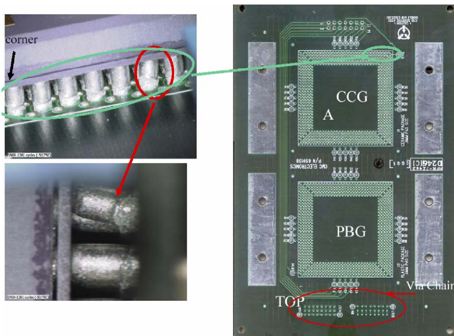
Fig. 11. Optical photomicrographs of CCGA built with a 10.5 mil thick stencil after 1138 cycles Cycle A ( -50/75^{\circ}\text{C} )—cracking from the package site rather than the board site commonly occurring.
